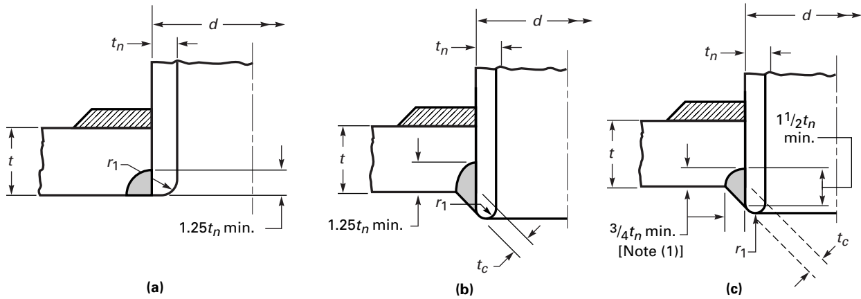
Figure NE-4244(d)-2 Partial Penetration Weld Connections
