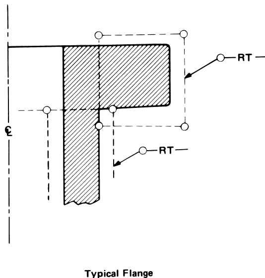
Figure NE-2575.2-1 Typical Pressure-Retaining Parts of Vessels (21)
