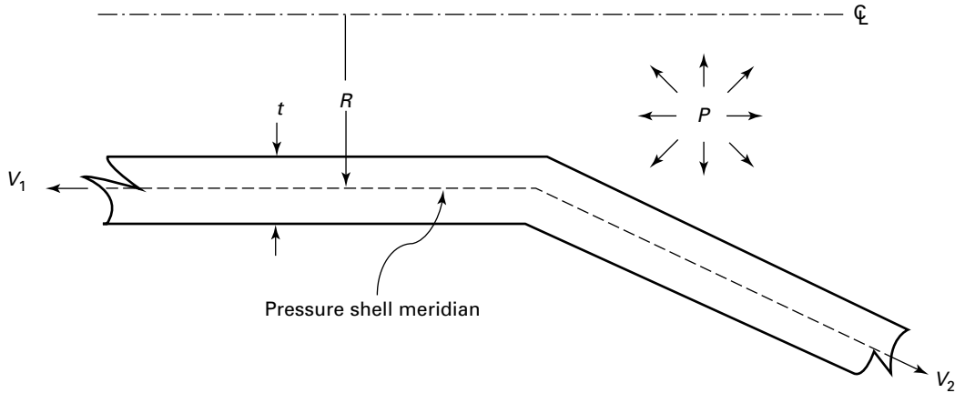
Figure NE-3213.10-1 Example of Acceptable Local Primary Membrane Stress Due to Pressure
