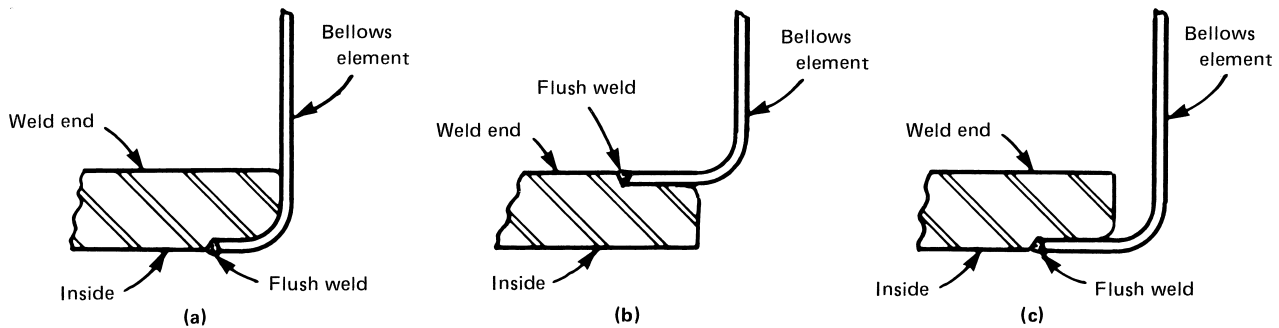
Figure NE-4810(c)-1 Bellows Attachment Welds
